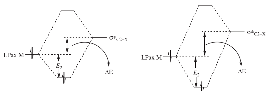
Fig. 2. Schematic representation of the correlation between the second order perturbation energies (i.e. stabilization energies E_2 ) and the energy gaps between donor and acceptor orbitals in conformations A and B of compounds 1–3.
