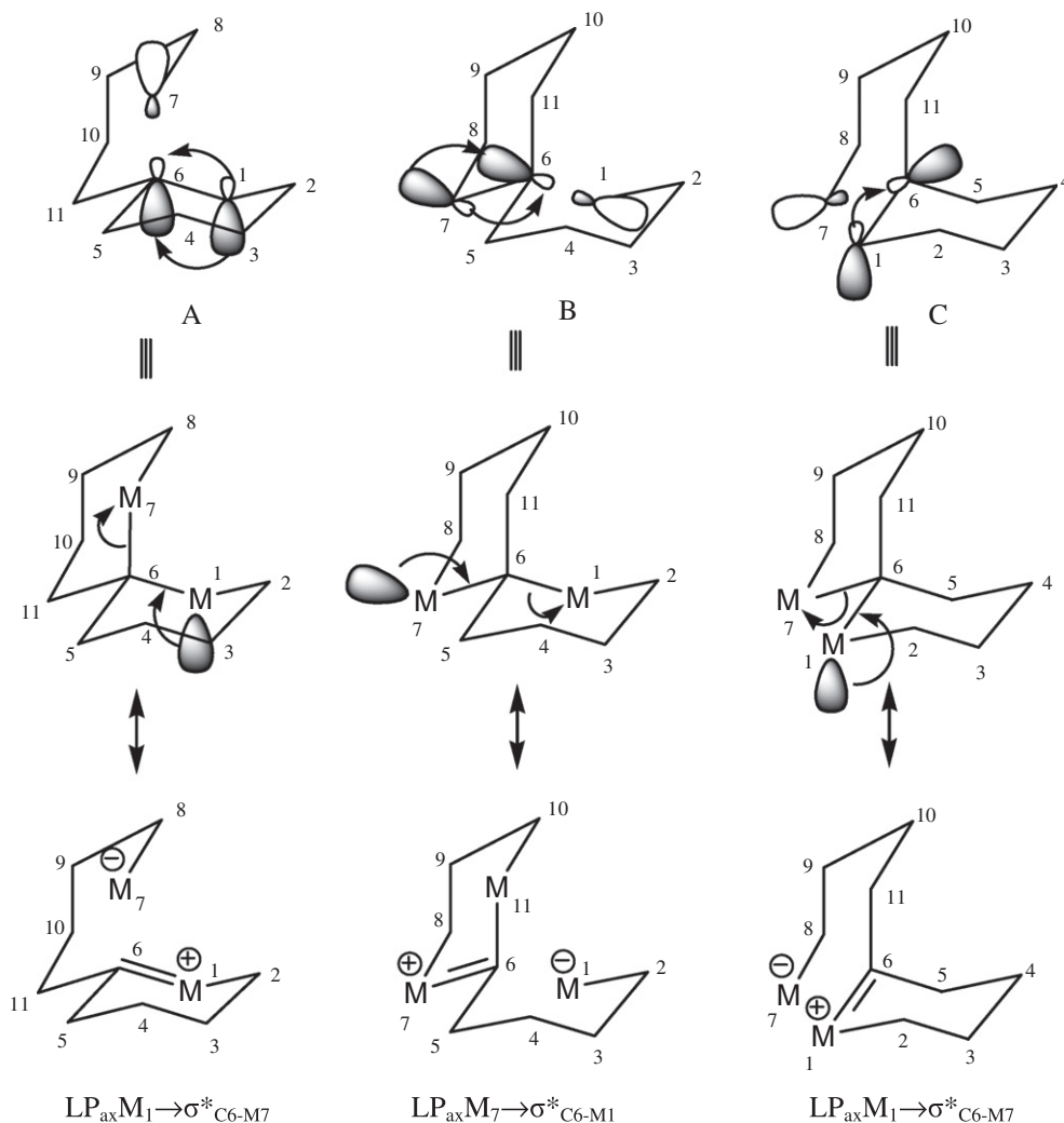
Fig. 1. Schematic representation of the electron delocalization between non-bonding and anti-bonding orbitals in conformations A, B and C of compounds 1–3.
