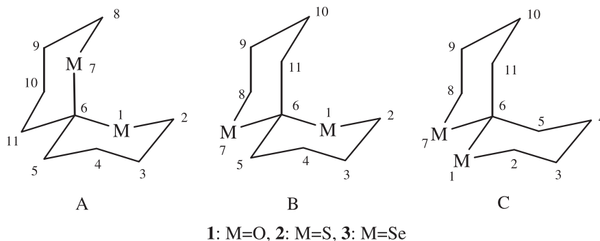
Scheme 1. Schematic representation of conformations of compounds 1–3.
