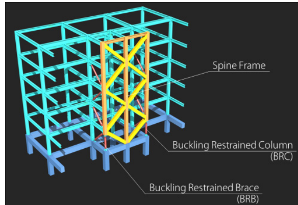
Fig.17 Structural system.[43]
