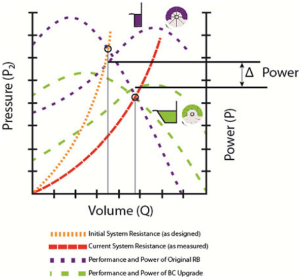
Fig. 2. Graphic representation of performance of original rotor to upgrade rotor.
