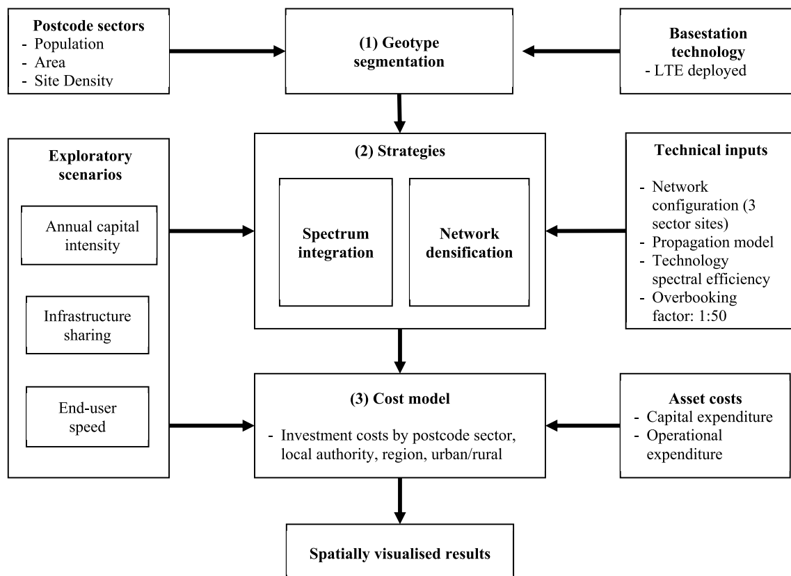
Fig. 1. Sequential methodology.
