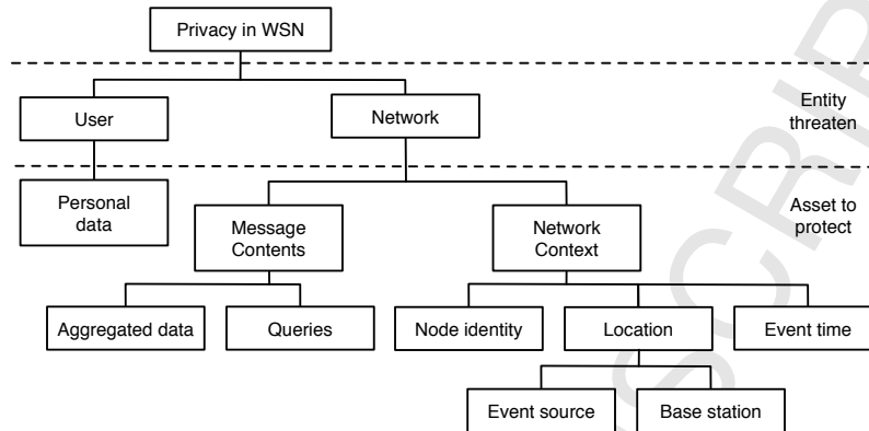
Figure 2: Privacy Problems in WSN
