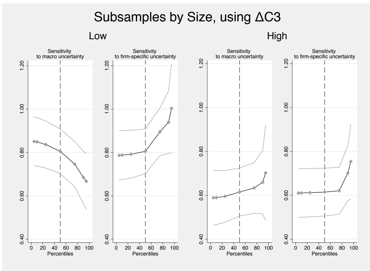
Figure 6: Sensitivity of marginal value of cash in subsamples
