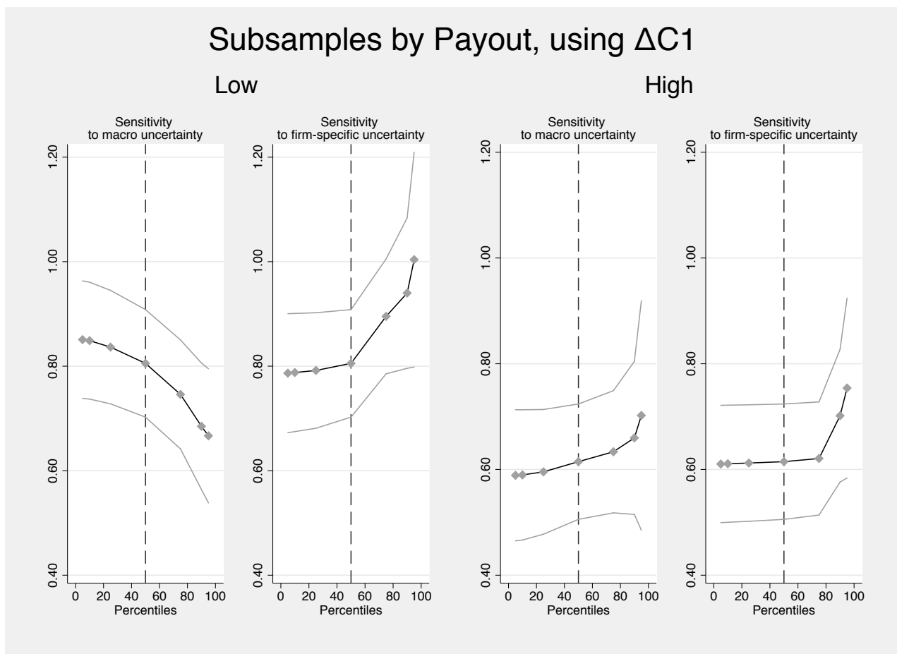
Figure 3: Sensitivity of marginal value of cash in subsamples
