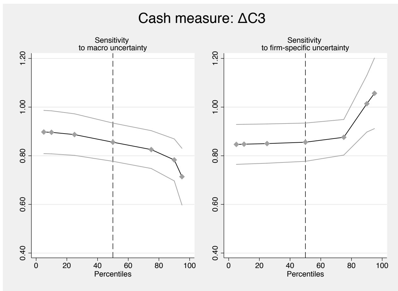
Figure 2: Sensitivity of marginal value of cash
