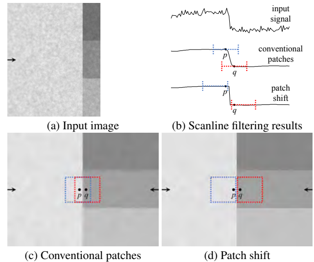
Figure 2: Patch shift. Conventionally, texture feature is computed in a patch centered at each pixel, in which case the patches for two adjacent pixels should have a large overlap, reducing the feature discriminability. In contrast, patch shift finds a nearby patch that stays clear of a prominent structure edge. (b) Filtering of the scanline marked by arrows. (c) Filtered by [Karacan et al. 2013]. (d) Filtered with patch shift. The results in (b) show that our approach preserves structure edges, unlike the conventional approach.
