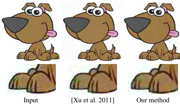
Figure 11: Cartoon JPEG artifact removal by [Xu et al. 2011] and our method.
