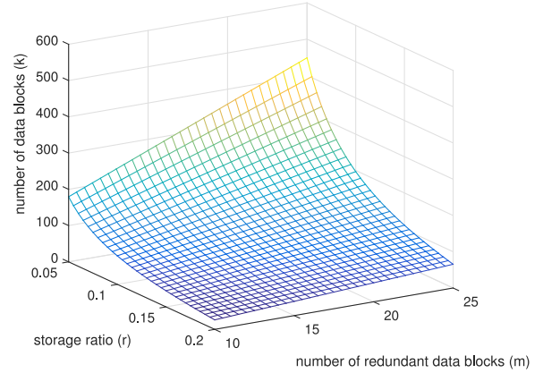
Fig. 7. Diagram of relationship of the number of data blocks ( k ), redundant data blocks ( m ) and storage ratio ( r ).
