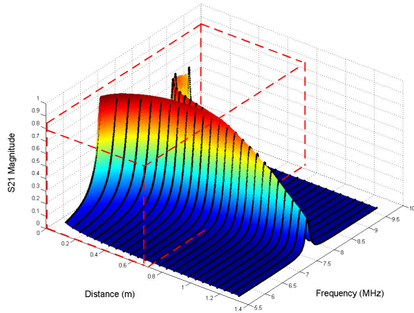
Fig. 7. Measured |S_{21}| data (black dots) plotted in magnitude form. Each row of black dots represents a frequency sweep taken by the VNA every 5cm as the receiver was moved away from the transmitter. The mesh underneath the data is the theoretical model.
