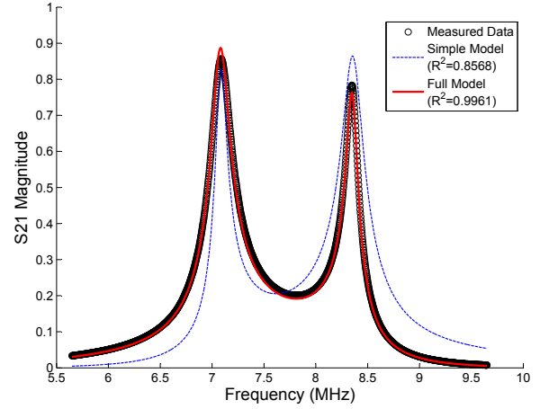
Fig. 6. Comparison of experimental data (black dots) to the simplified transfer function (dotted blue line), and to the complete transfer function (red line). The simple model neglects parasitic cross coupling (e.g. k_{13}, k_{24}, k_{14} ) and does not reproduce the amplitude difference between the upper and lower modes. The complete model reproduces this amplitude difference, which is explained by the phase of the parasitic coupling terms ( k_{13}, k_{24} ) relative to the non-parasitic terms (e.g. k_{23} ) for the two resonant modes.
