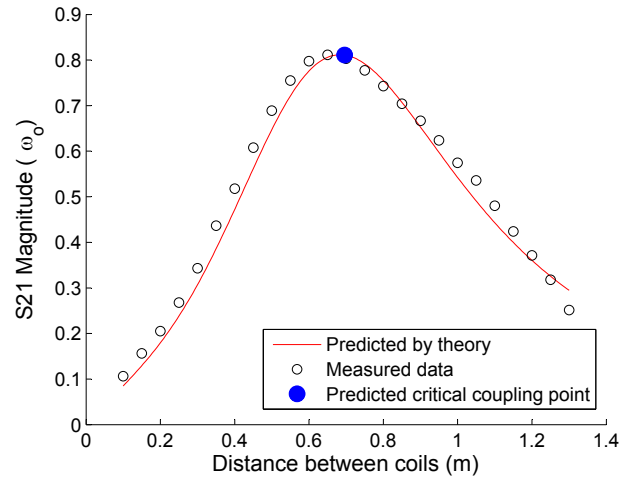
Fig. 9. Predicted behavior of the wireless power system at the resonant frequency f_o using Neumann's formula along with the predicted critical coupling point (blue dot) and S_{21} measured data.
