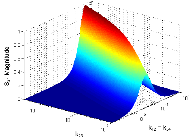
Fig. 14. |S_{21}| as a function of k_{23} and k_{12} .
