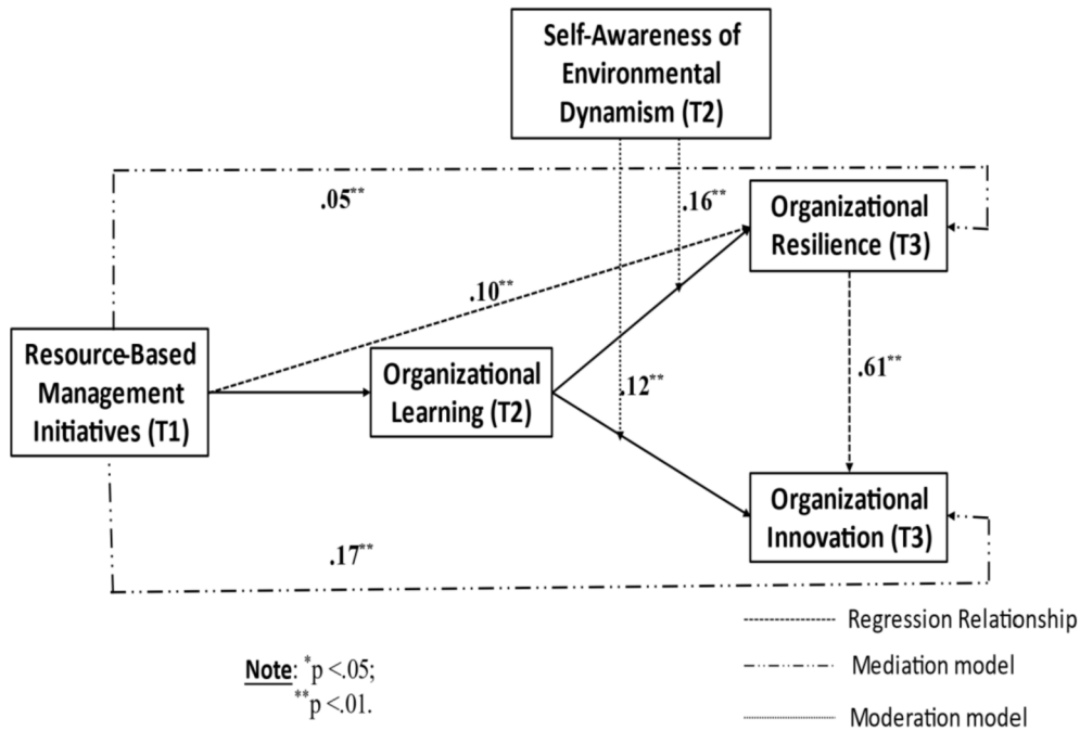
Fig. 2. Results of path analysis.
