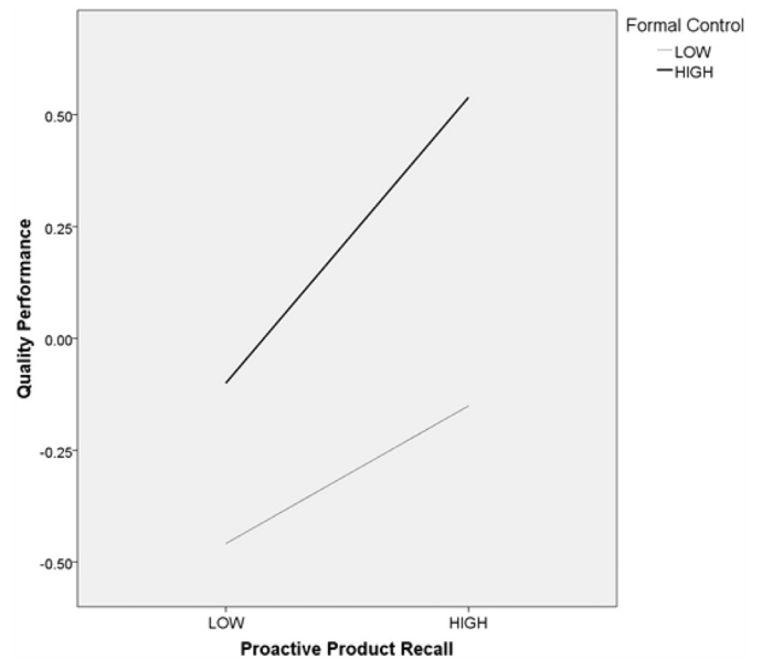
Fig. 5. Moderating effect of FC on relationship between RCR and QP.
