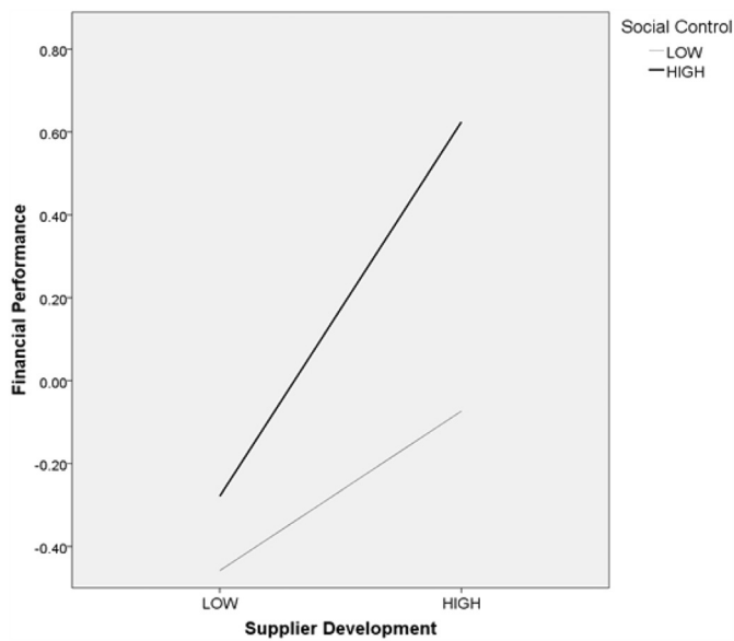
Fig. 6. Moderating effect of SC on relationship between SD and FP.
