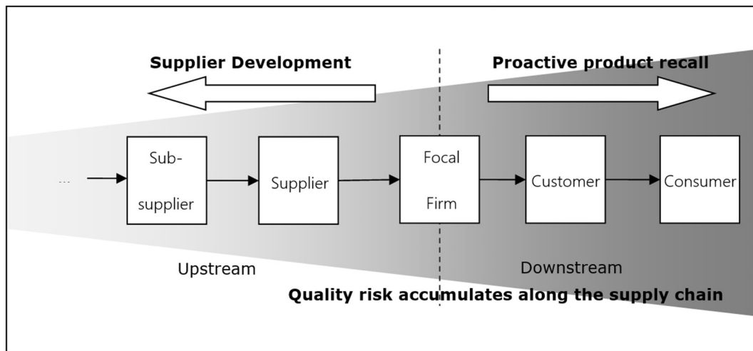
Fig. 2. SD and PPR adopted in firm's supply chain.
