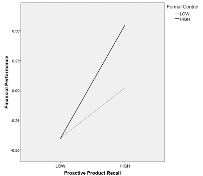
Fig. 4. Moderating effect of FC on relationship between RCR and FP.
