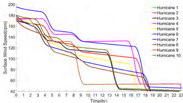
Fig. 11. The surface wind speed variations of 10 different hurricanes
