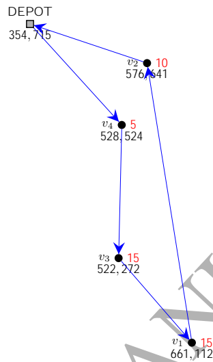
Figure 1: Small example with four customers randomly scattered in [0, 1000]^2 .
