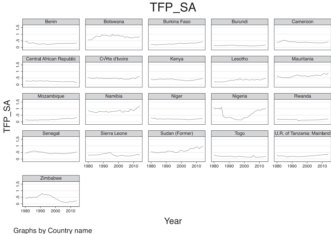
Fig. 1. TFP superlative index number, country of reference South Africa (TFP_SA).
