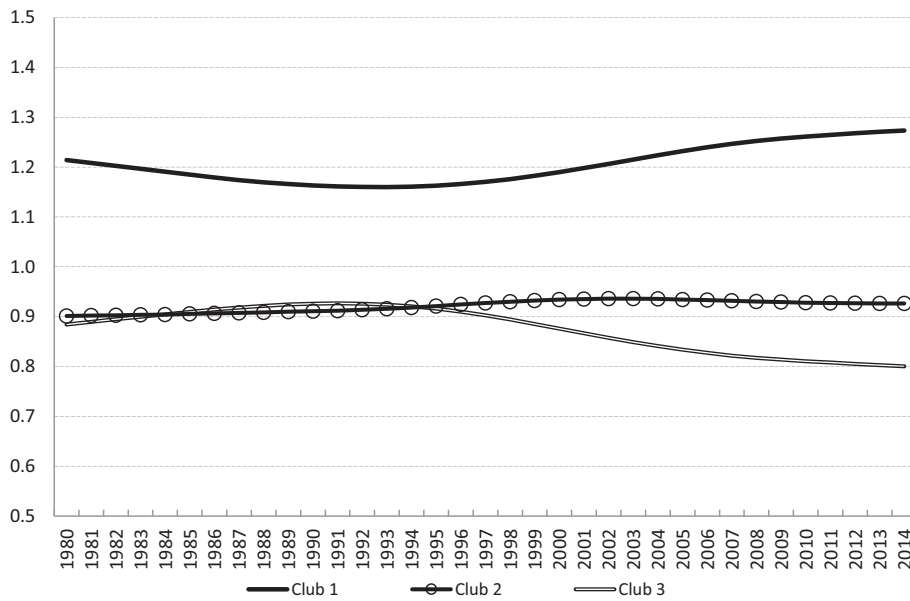
Fig. 4. Relative transition paths across clubs based on the TFP level relative to the regional leader South Africa (1990–2014).
