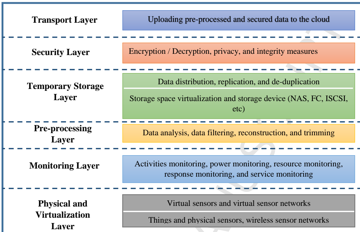
Figure 2. Fog Computing Architecture
