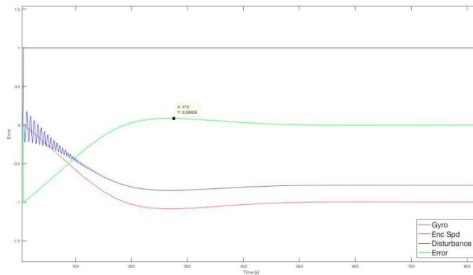
Fig.5. Used Intelligent PID Controller
