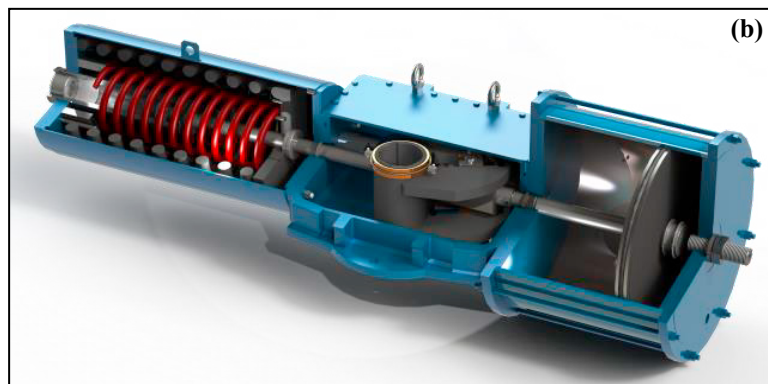
Figure 1: (a) LPS-30 actuator mounted on TMBCV Valbart valve, (b) Single acting fail close heavy-duty pneumatic actuator
