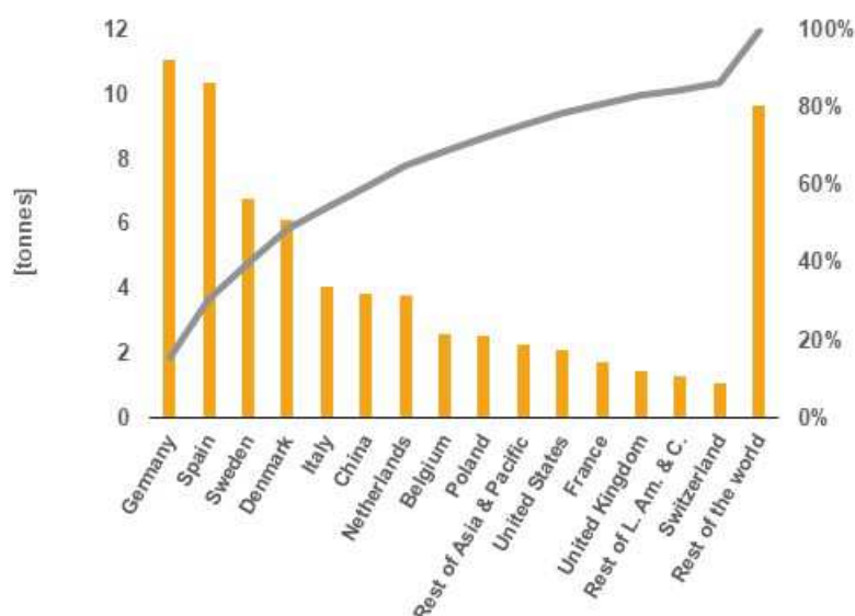
Figure 6: Use of veterinary medicines per producer country (yellow bars). Grey line shows cumulative results.
