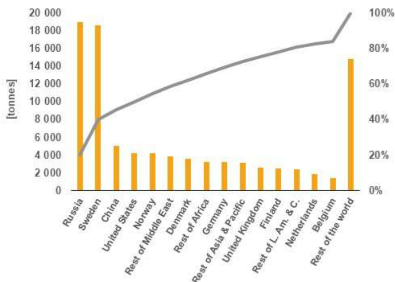
Figure 8: Emissions of hazardous substances per producer country (yellow bars). Grey line shows cumulative results.
