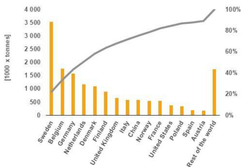
Figure 2: Use of hazardous chemical products per producer country (yellow bars). Grey line shows cumulative results.
