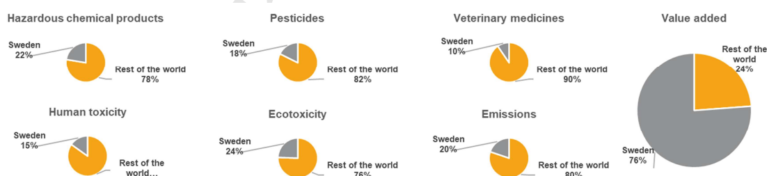
Figure 11: Share of use, emissions, and potential impact in Sweden vs outside Sweden across all indicators and compared to the share of the consumption as contribution to the Gross Domestic Product (Value added).
