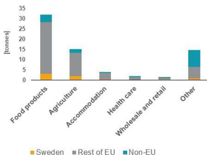
Figure 7: Use of veterinary medicines per product group. The results are presented comparing Sweden, the rest of the EU (plus Norway and Iceland) and non-EU.
