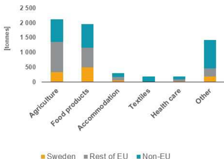
Figure 5: Use of pesticides per product group. The results are presented comparing Sweden, the rest of the EU (plus Norway and Iceland) and non-EU.
