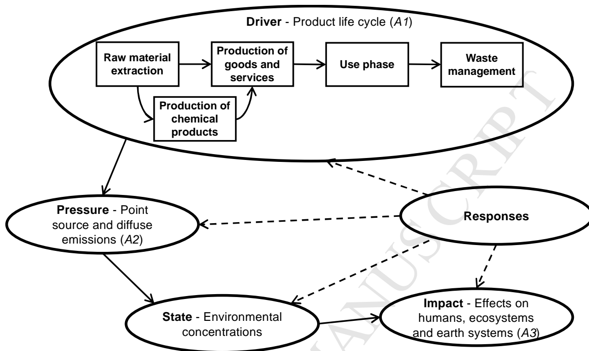
Figure 1: Physical flows of chemicals shown with solid arrows in a life-cycle perspective and in relation to the driver-pressure-state-impact-response framework (DPSIR), with societal responses shown with dashed arrows. A1-3 refers to the different aggregation methods.
