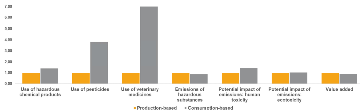
Figure 12: Consumption-based versus production-based indicators across all indicators (normalized to production-based=1), including the contribution to the Gross Domestic Product (Value added).
