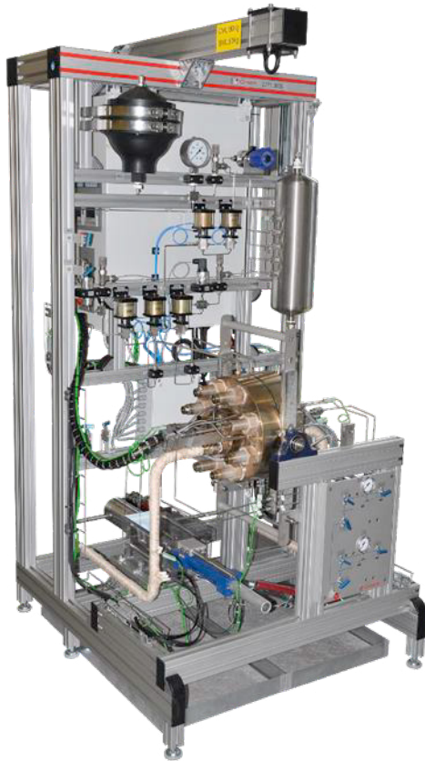
Figure 7: View of the fatigue new bending device FABIME2E
