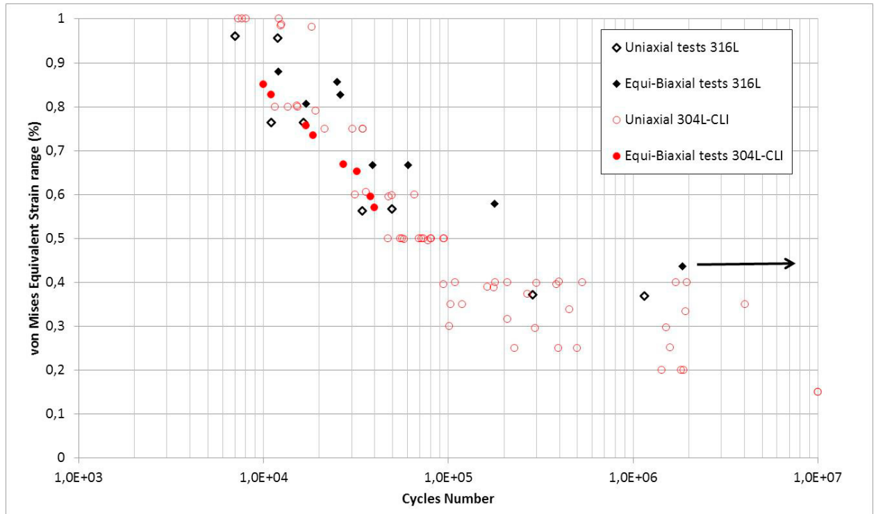
Figure 5: Fatigue data obtained on the two austenitic stainless steels (316L and 304L-CL1)
