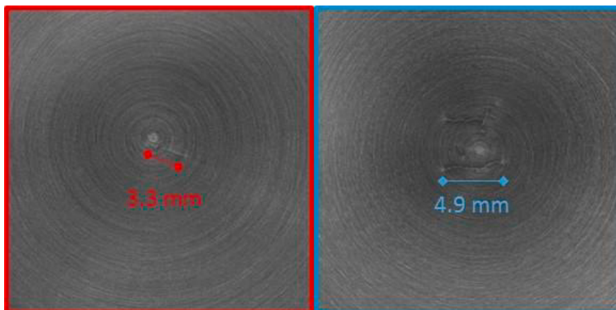
Figure 9: View of the fatigue crack initiation when the pressure criterion is goal taken into account
