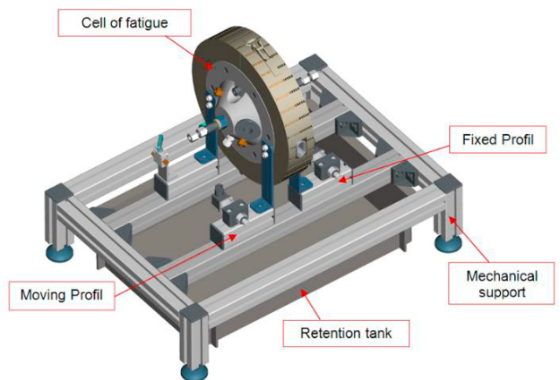
Figure 4: View of the spherical bending device: fatigue cell
