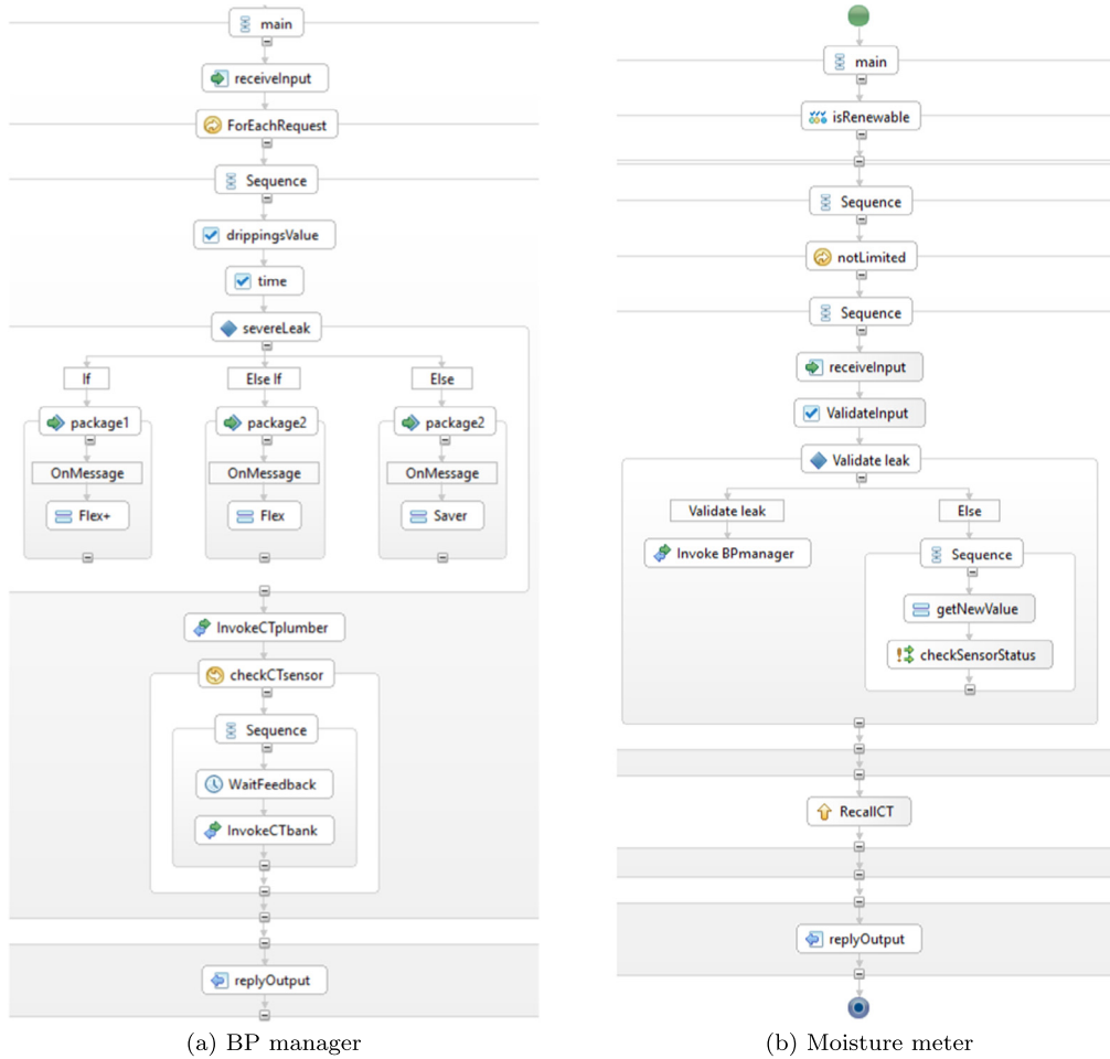
Fig. 12. BPEL specification.
