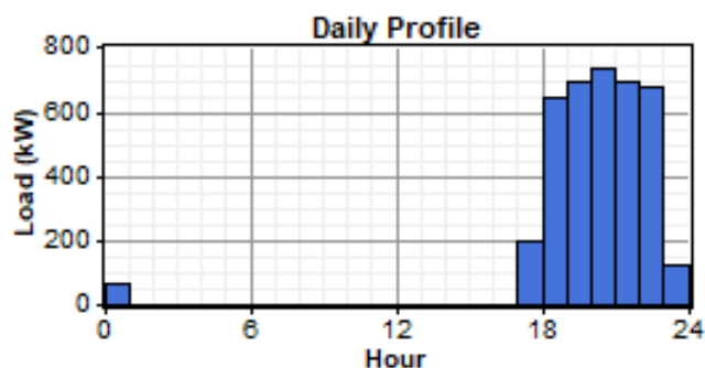
Fig. 3. Daily load variation of lights
