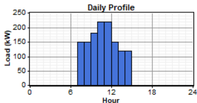
Fig.4 Daily load variation of socket.
