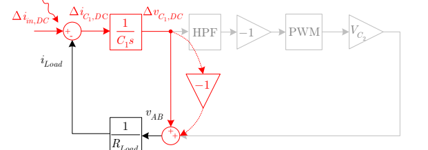
(a) Introduction of voltage feed-forward.
