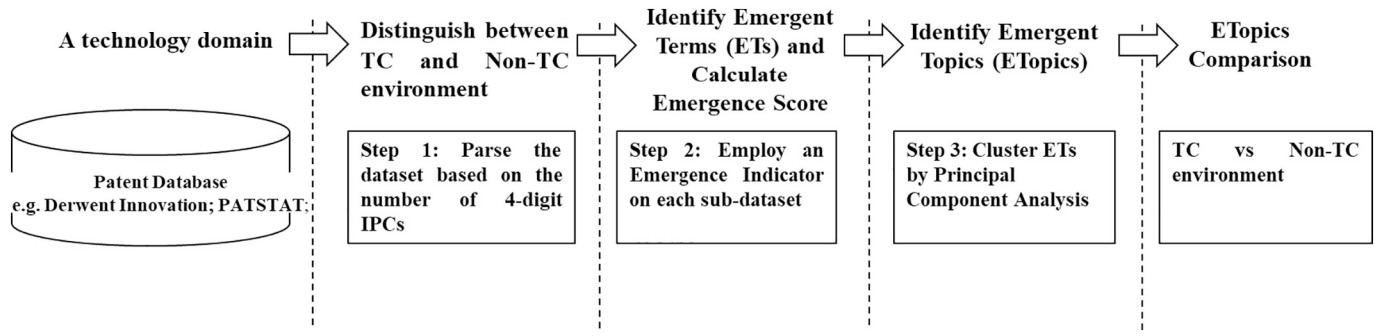
Fig. 1. Overall process to generate emergent terms in relation to technological convergence.
