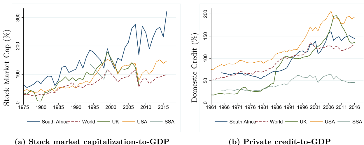
Fig. 1. Institutional context.
