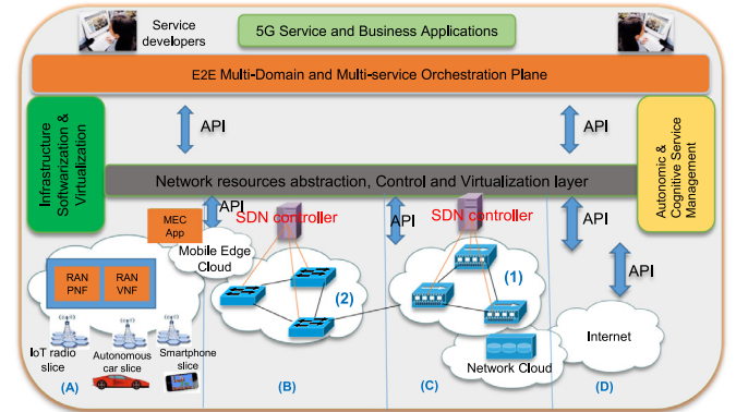
Fig. 4. Software network technologies in 5G architecture. A indicates RAN; B = transport networks; C = core networks and D represents the Internet.
