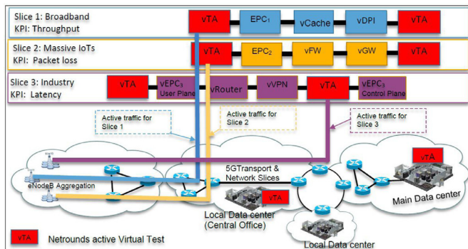
Fig. 20. Three network slices with different critical key performance indicators. The Massive IoT slice may include VNFs like vEPC, vFW, and vGW. Packet loss is the KPI to meet SLA requirements for this slice. The industry slice may include VNFs such as vRouter and vVPN. Latency is the KPI for this slice to meet SLA requirements [210].
