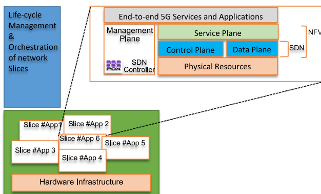
Fig. 25. 5G!Pagoda slice template and instantiated slices.
