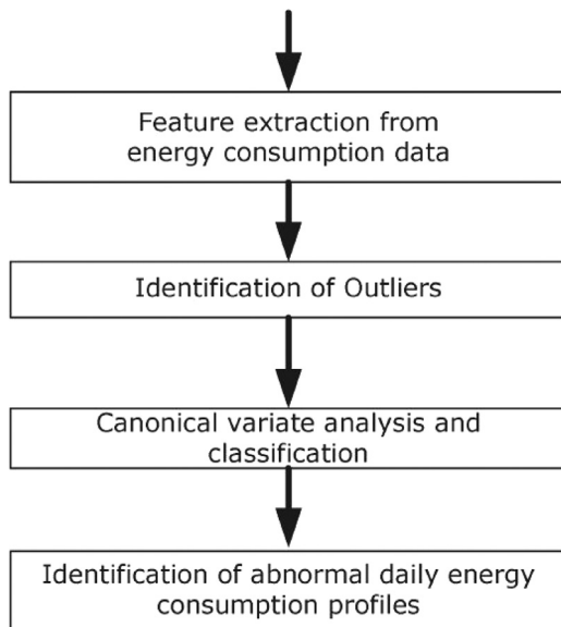
Fig. 8. Outline of the identification of outliers and modeling of the daily energy consumption profiles [67].
