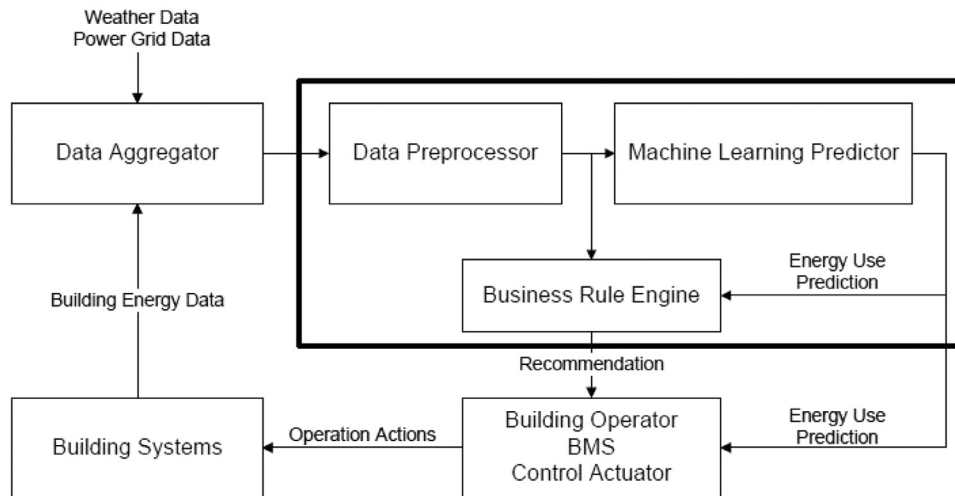
Fig. 7. Predictive building energy optimization workflow [65].
