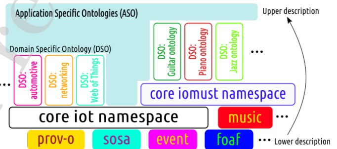
Figure 3: The IoMusT Ontology is built up incrementally leveraging lower level concepts. It provides the base for other Domain Specific Ontologies (DSO) and other Application Specific IoT ontologies (ASO).
