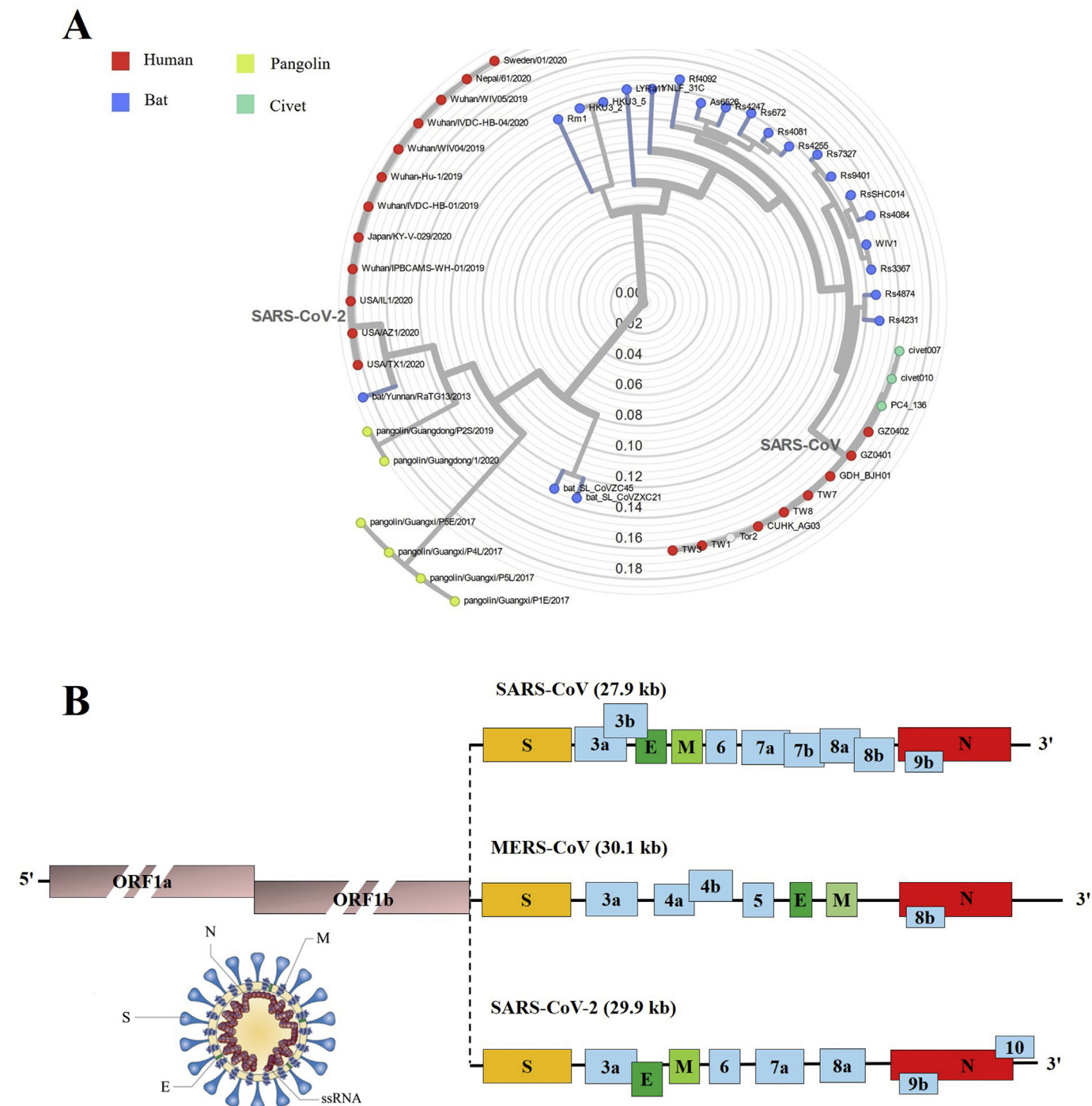
Fig. 1. The phylogenetic tree of SARS-like coronaviruses complete genome sequences and genome of SARS-CoV, MERS-CoV and SARS-CoV-2.
