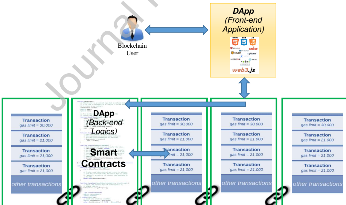
Figure 11: DApp and smart contracts in the blockchain network
