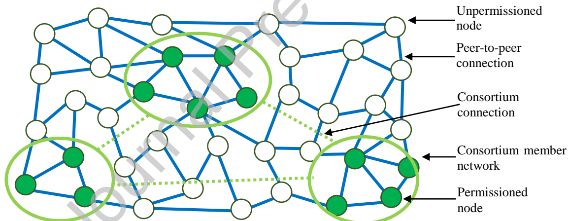
Figure 9: Skeleton of a consortium blockchain network
