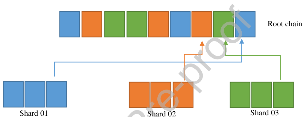
Figure 7: Blockchain network with Shards
