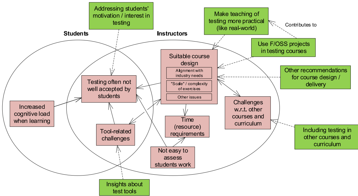
Fig. 21. Relationship among challenges and insights presented in the papers (green-backed rectangles are insights and pink-backed rectangles are challenges).
