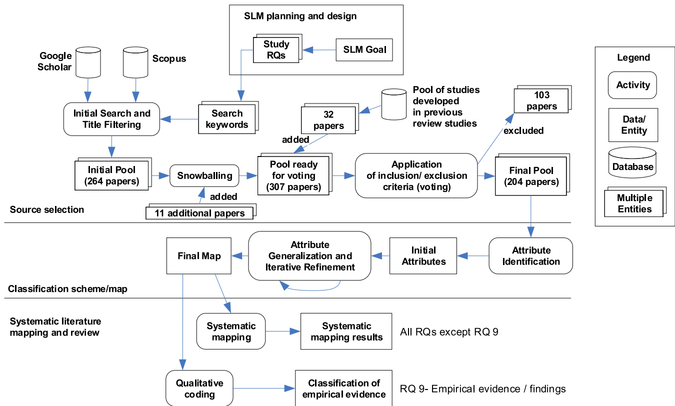
Fig. 3. An overview of SLM process (represented as a UML activity diagram).
