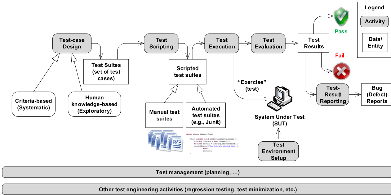
Fig. 12. Overview of a typical software test process and its activities (from (Garousi and Pfahl, 2016)).
