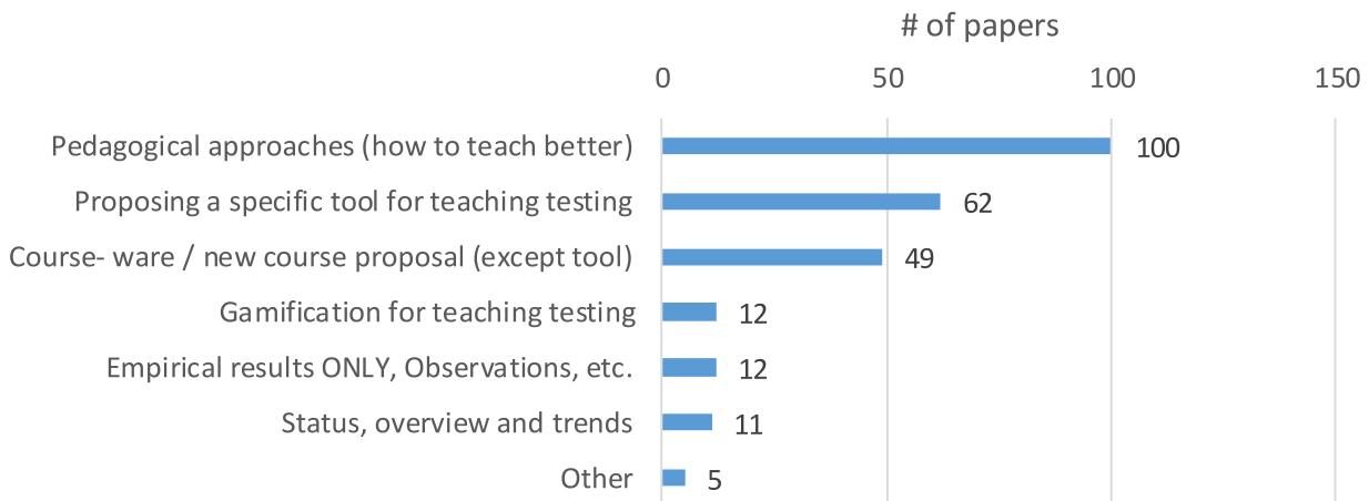
Fig. 8. Classification of studies by contribution types.
