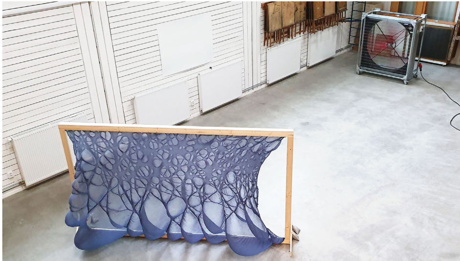
Fig. 7 Wind-machine set-up for the larger drop-stitch sample described in Section 4.4.
