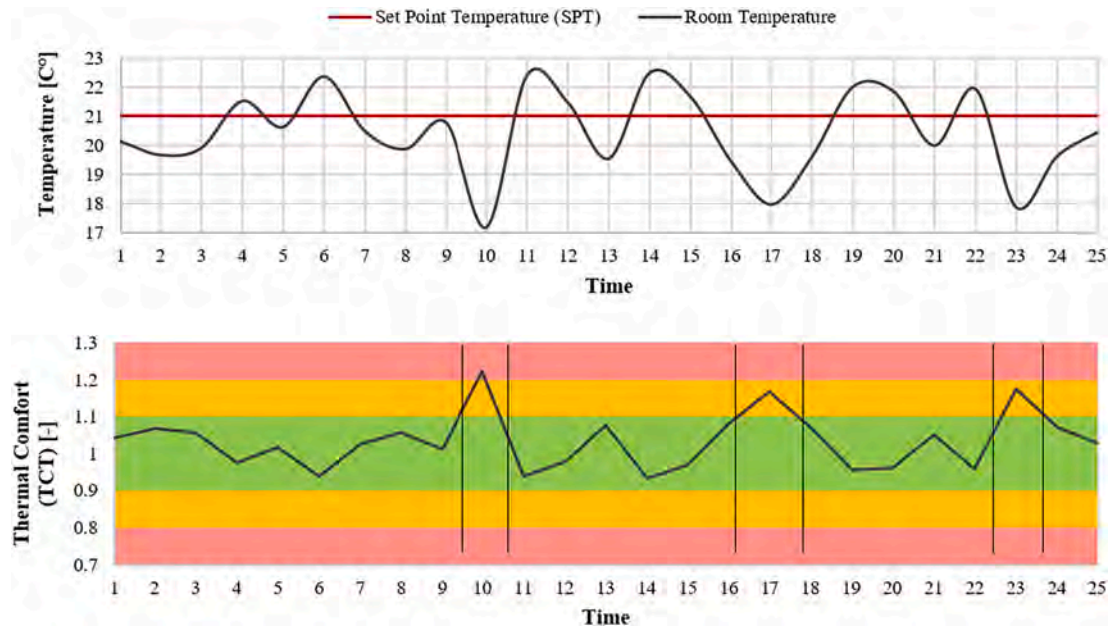
Fig. 6. Exemplary visualization of performance assessment for the temperature thermal comfort ( TC_T ). For a given SPT of 21 °C and the measured room temperature values (a), the TC_T ratio must stay within the defined range (green), causing a reduced reward (orange) or failure (red) for the facility manager when deviating (b). (For interpretation of the references to colour in this figure legend, the reader is referred to the web version of this article.)
