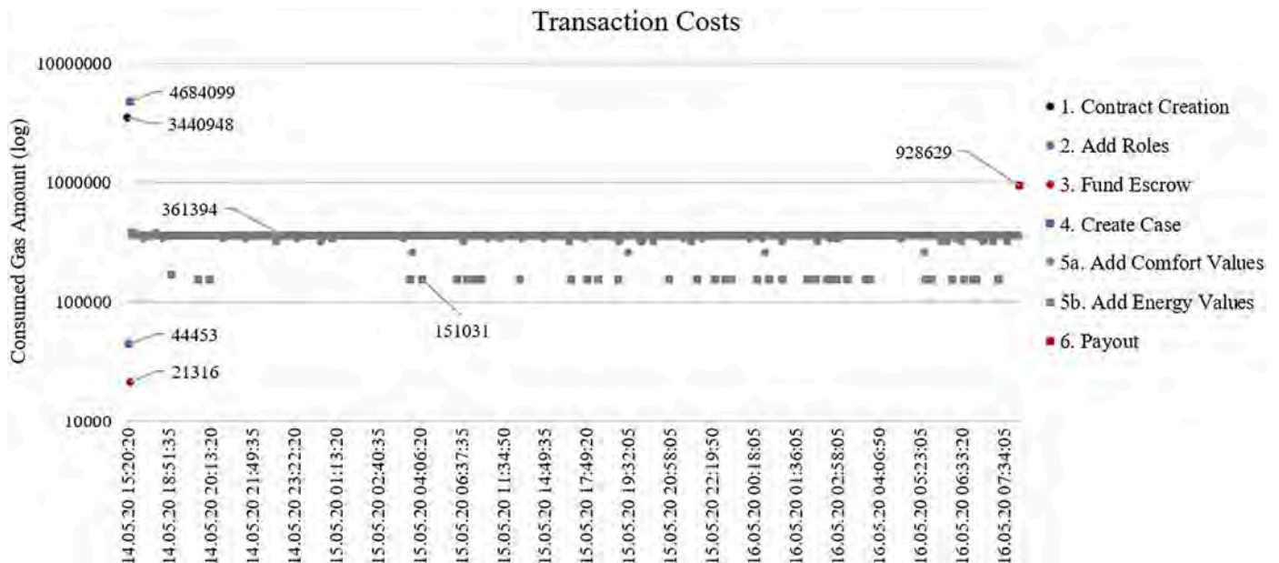
Fig. 11. Transaction costs (Gas) for the executed transactions of the test case.
