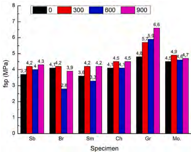
Fig. 23. Effect of freeze-thaw cycles on splitting tensile strength of composite specimen ( f_{sp} =splitting tensile stress, Sb = sandblasted; Br = Brushed; Sm = smooth; Ch = chipped; Gr = grooved; Mo = monolithic (only concrete)) [127].
