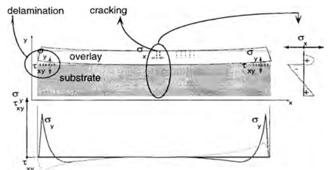
Fig. 20. Damage mechanisms in strengthening systems [82,118].
