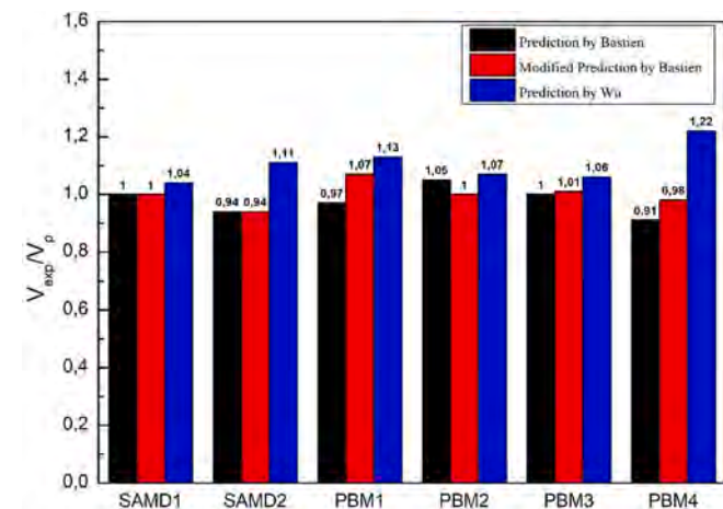
Fig. 7. Comparison of punching shear strength between experimental and predicted results [56,58,59]. (Note: V_{exp}/V_p indicates the ratio between experimental and predicted results, and the series of SAMD samples were tested by Wuest [71], and the series of PBM sample were tested by Bastien [56].).
