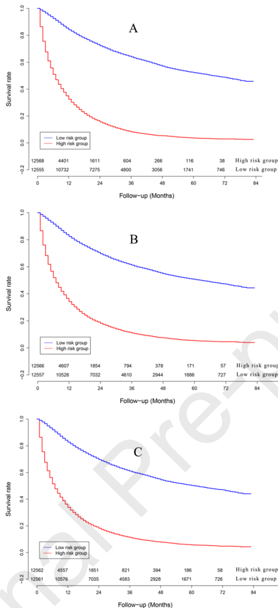
Figure 4. Survival curves of high risk patients and low risk patients in model cohort: (A). Random survival forest; (B). Multi-task logistic regression; (C). Cox survival regression.
