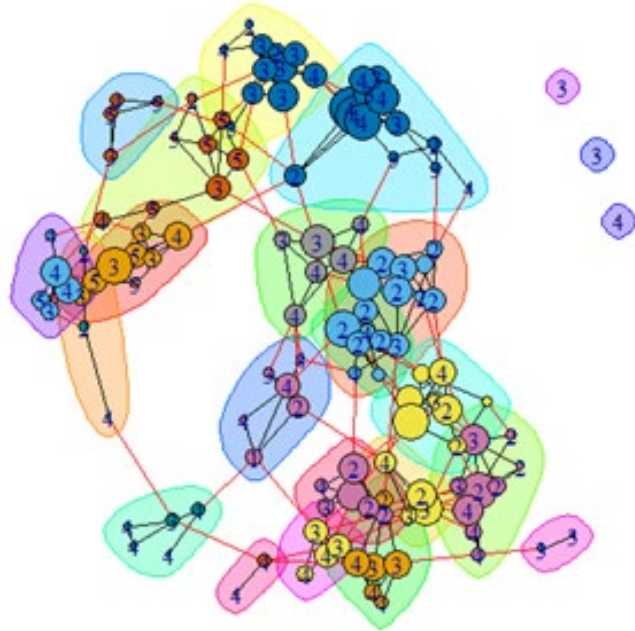
Figure 8: Community Detection using Label Propagation.
