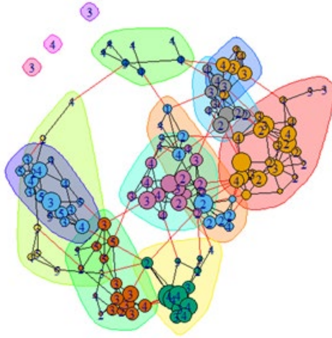
Figure 2: Community detection using Fast Greedy.
