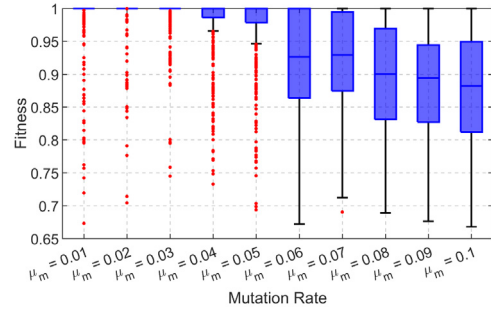
(b) Fitness score distribution over generations
