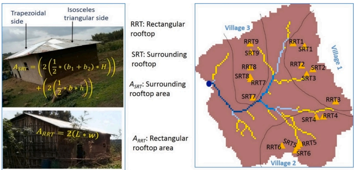
Fig. 3. Designs of experimental rooftops and their locations at the Debre Mawi.
