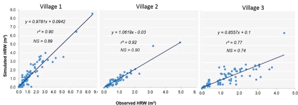
Fig. 11. Comparison of the observed and simulated amounts of harvested rooftop water (HRW) for the rainy period (15/6/2016–23/10/2016).
