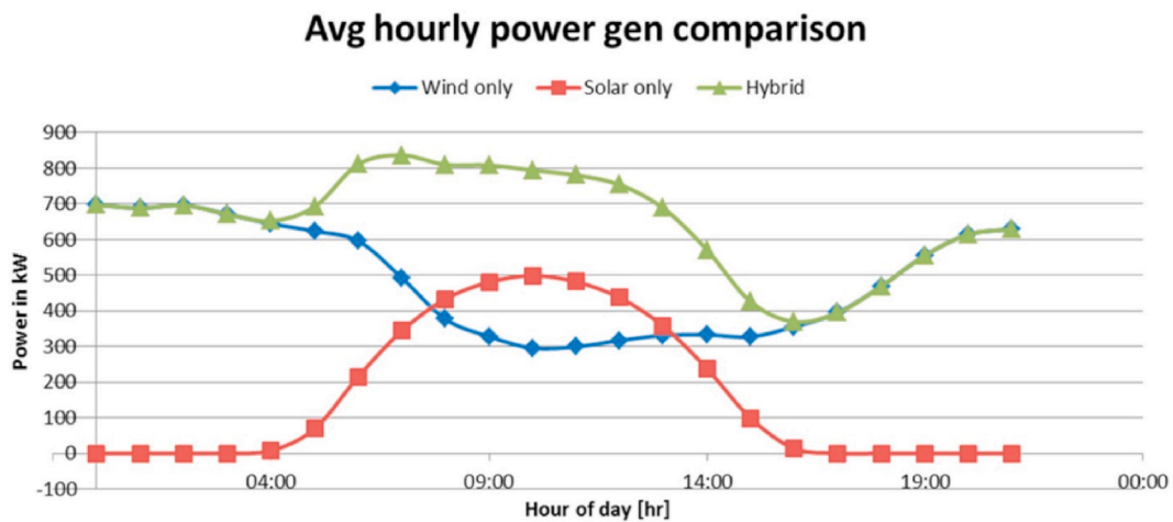
Fig. 9. Power generation of a 1.5 MW wind turbine, 750 kWp, and the hybrid system [87].
