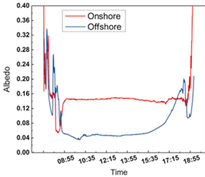
Fig. 4. Comparison of onshore and offshore albedo in Singapore [55].
