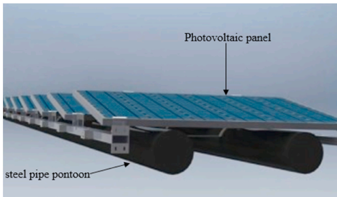
Fig. 11. Example of a steel pipe pontoon system for floating photovoltaics [102].
