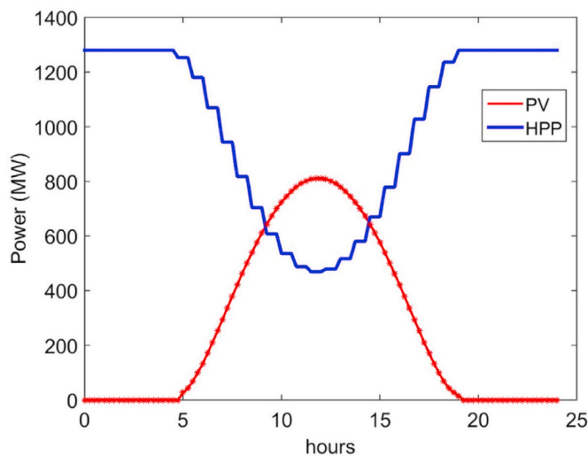
Fig. 7. Hydropower plant and floating photovoltaic power in MW across a summer day for the Longyanxia plant [75].
