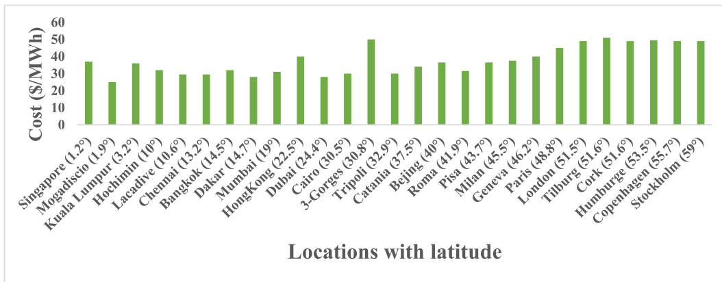
Fig. 5. Cost of solar energy production from 1 MWh FPV system according to the latitude and longitude.
