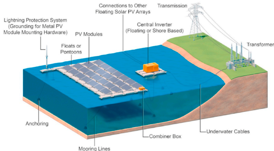
Fig. 1. Example of a standalone floating photovoltaic system, adapted from [15].
