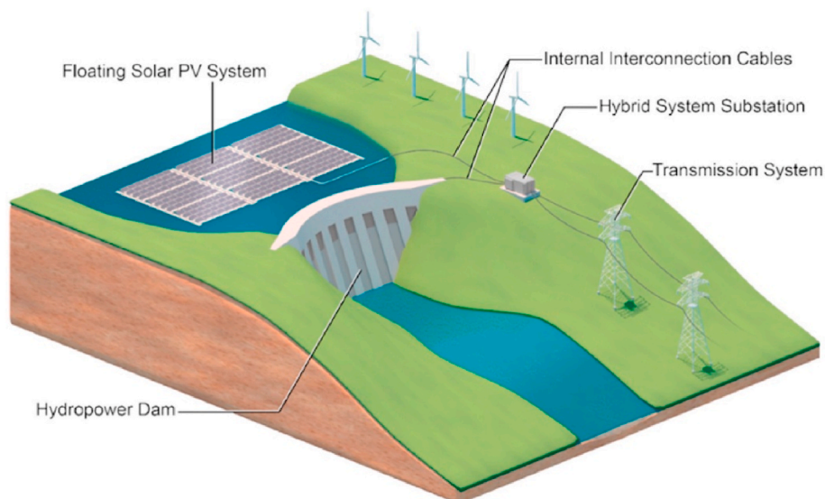
Fig. 6. Schematic of floating photovoltaic-integrated hydropower plant, adapted from [15].
