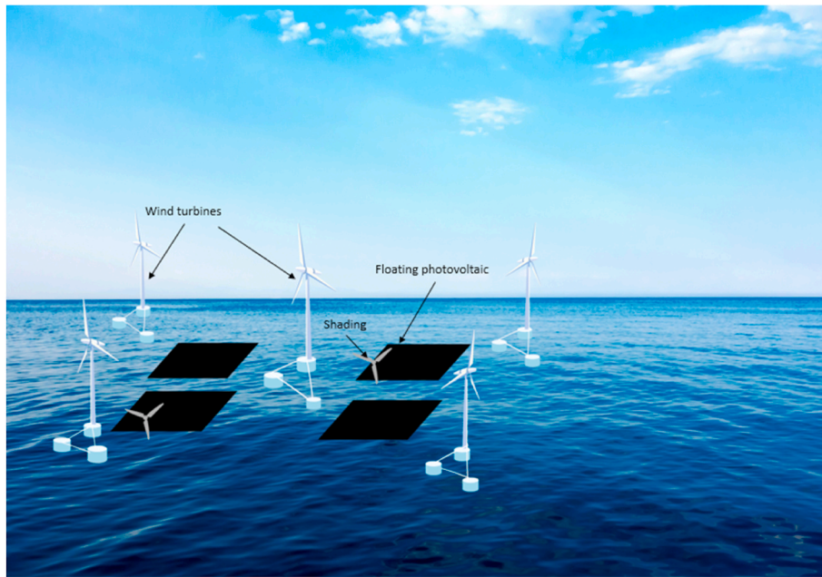
Fig. 8. An example of the possible layout for an offshore wind farm integrated with floating photovoltaics.
