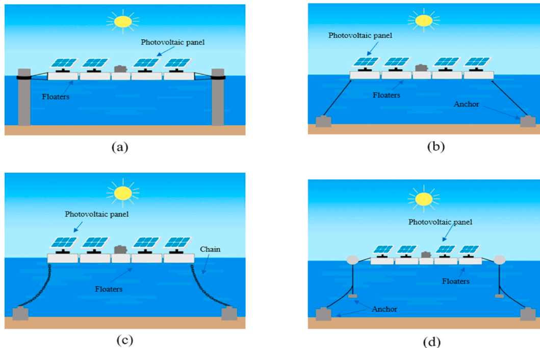
Fig. 3. Schematics showing the different possible mooring systems for floating photovoltaic systems. (a) Rigid mooring system, (b) Taut mooring system, (c) Catenary mooring system and (d) Compliant mooring system.
