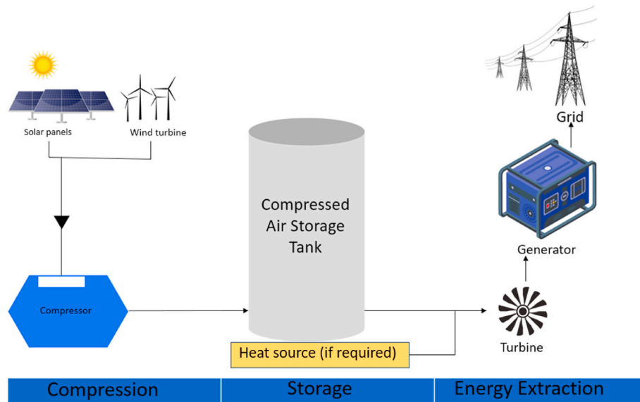
Fig. 10. Schematic of the compressed air energy storage system process.
