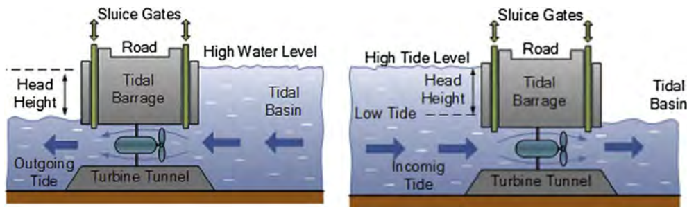
Fig. 2. The function of tidal barrage technology.
