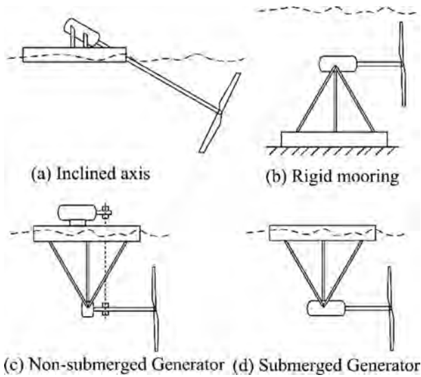
Fig. 3. Horizontal axis turbines.
