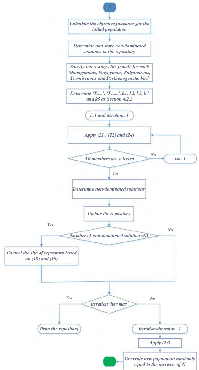
Fig. 9. Flowchart of the proposed MMOBMO algorithm.
