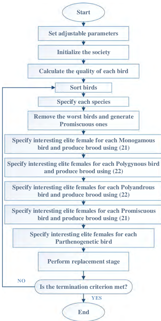
Fig. 7. Flowchart of BMO algorithm [32].
