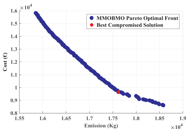
Fig. 21. Pareto solutions of the proposed MMOBMO algorithm for the second test MG.
