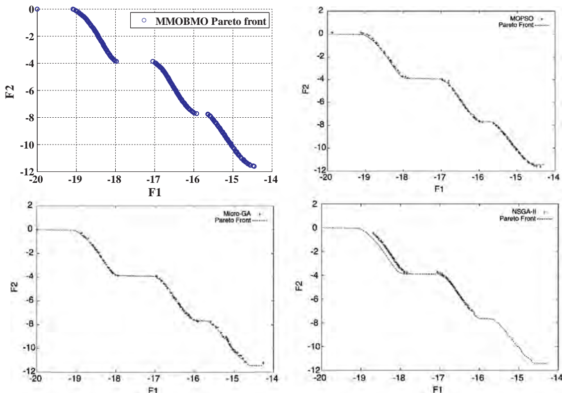
Fig. 10. Comparison between the Pareto front of the proposed MMOBMO and results of [50] for Test Function 1.
