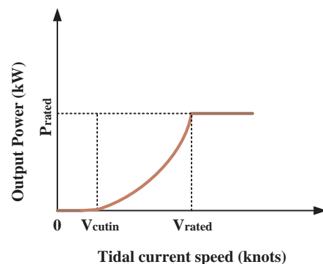
Fig. 5. Speed-power characteristic of TST [30].
