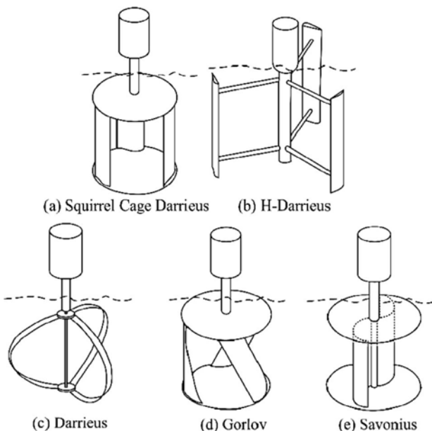
Fig. 4. Vertical axis turbines.
