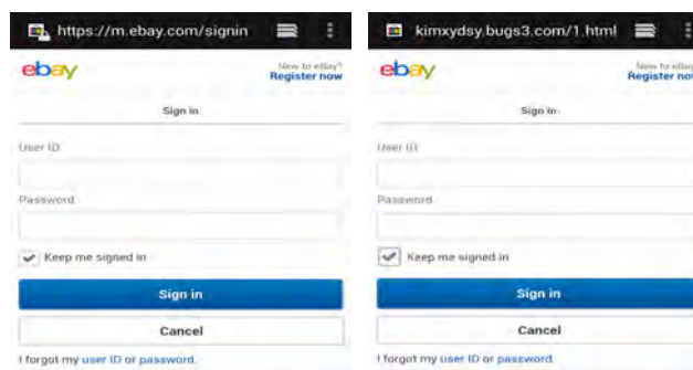
(a) Ebay Official Login Page (b) Ebay Phishing Login Page
