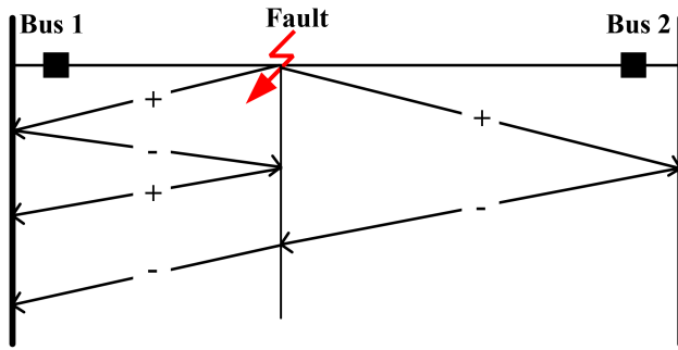
Fig. 2 Protection using travelling waves [75]
