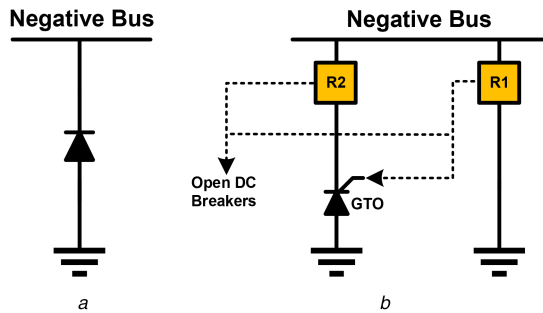
Fig. 3 Structures of reconfigurable grounding systems (a) Diode-grounded system, (b) Thyristor-grounded system
