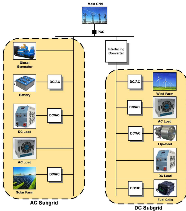
Fig. 1 Architecture of a typical hybrid AC/DC microgrid
