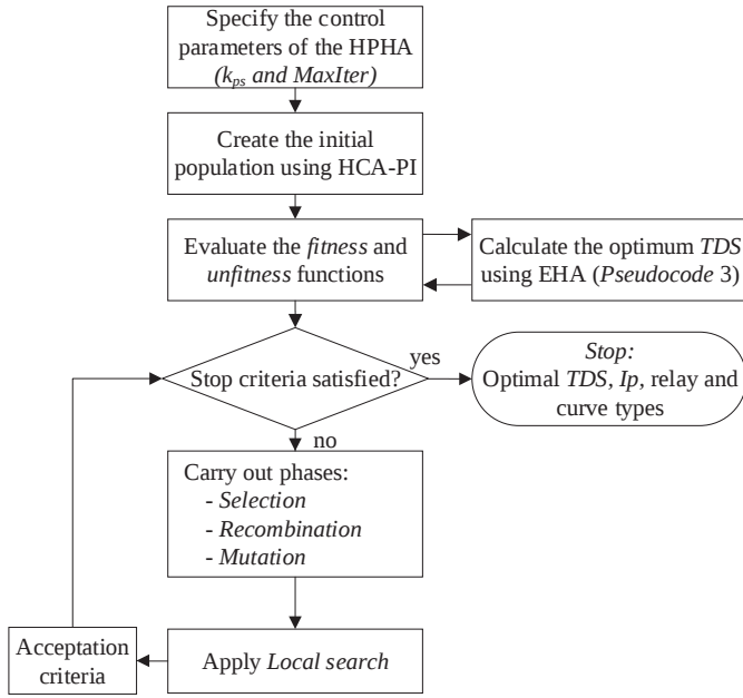
Fig. 2. Flowchart of the proposed HPHA.
