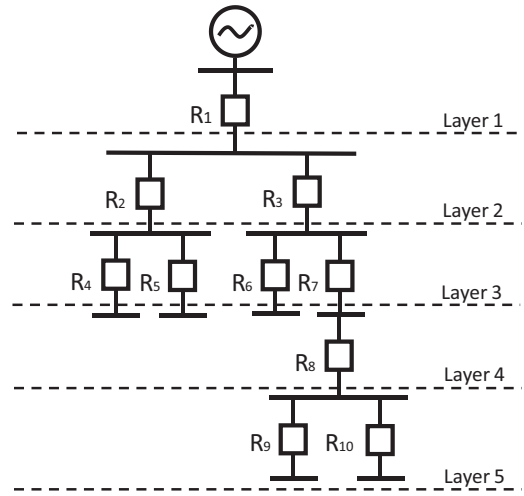
Fig. 4. OCRs renumbering in a RDN (test system II).
