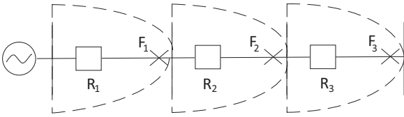
Fig. 1. Radial system with three relays and their respective primary protection zones.
