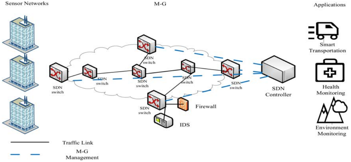
Fig. 4. Dataflow streams.
