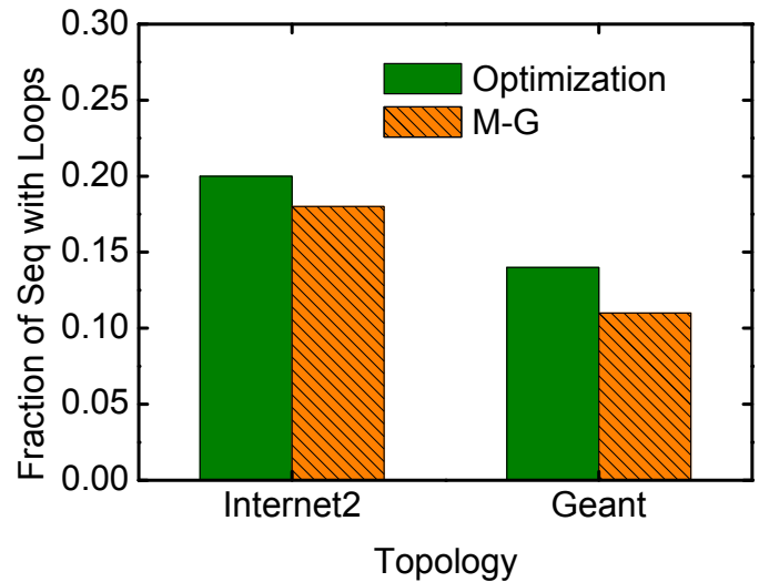
Fig. 16. Fraction of sequences with loops.
