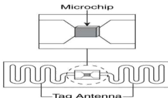
Fig. 9 Components of semi-passive/semi-active tag
