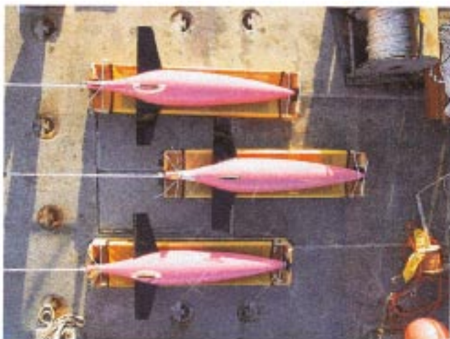
Fig. 1. Top view of three Seaglider vehicles in their handling cradles on deck. Plastic tubing is connected to the conductivity cell mounted atop the pink fairing just aft of its maximum diameter between the wings on two of the three vehicles. The white antenna masts extend aft of the fairings outside the view of this image.
