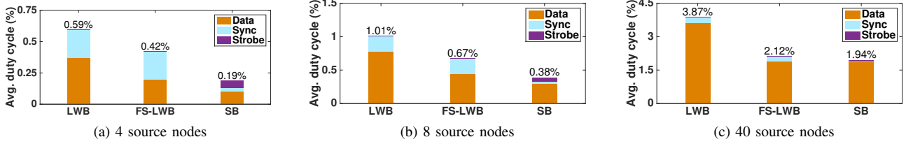
Fig. 9: Experiments on Indriya with 80 nodes: average radio-on time for nodes for various operations of Sleeping Beauty (SB).
