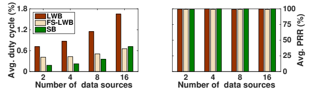
Fig. 8: Experiments on FlockLab: average duty cycle per node over a long period and average packet reception ratio.
