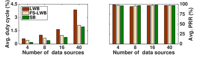
Fig. 7: Experiments on Indriya: average duty cycle per node over a long period and average packet reception ratio.
