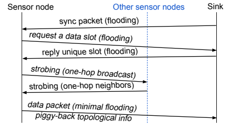
Fig. 2: Conceptual overview of Sleeping Beauty.
