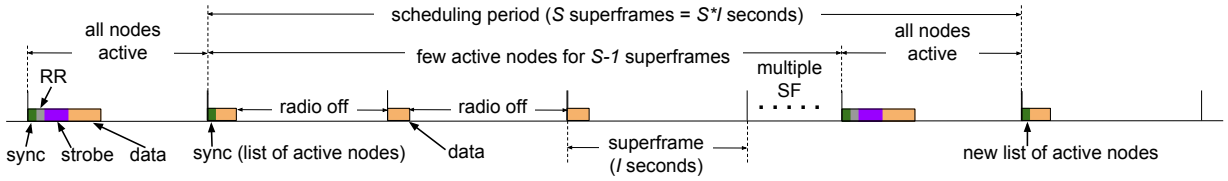
Fig. 4: Periodic strobe slots and new set of active node dissemination using various superframe structures in the steady state.
