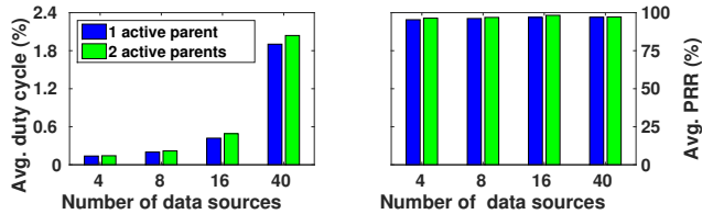
Fig. 11: Comparison of average radio-on time and PRR when one and two parent nodes are selected active.
