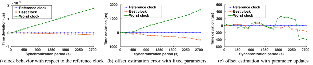
Fig. 6: Behavior of two clocks (best and worst) with respect to the reference clock.
