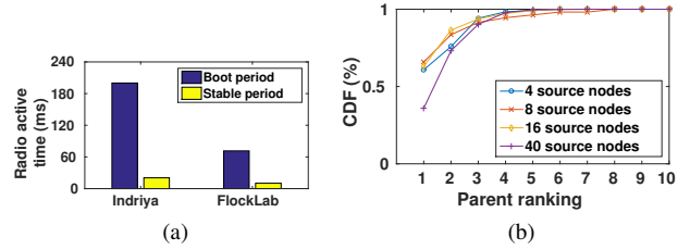
Fig. 10: (a) Strobe overhead during bootstrapping and steady state. (b) Active parent distribution across the ranked list.
