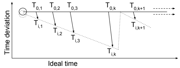
Fig. 5: Aperiodic one-way communication between sink (solid line) and sensor node (dotted line), and the effect of iterative clock correction at the sensor node at the k^{th} time instant [19].
