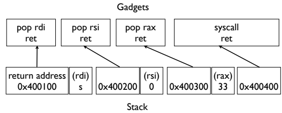
Figure 3. ROP chain for dup2(s, 0). The system call number needs to be in rax and dup2 is system call #33. Arguments are passed in rdi and rsi . Because the attacker already controls the stack, pop gadgets are used to load registers from values on the stack.
