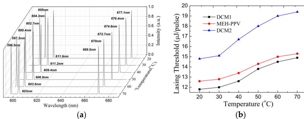
Figure 6. Tuning property for the tri-wavelength lasing HPDLC DFB laser by elevating temperature. (a) Dependence of the lasing spectra to operation temperature. (b) The working lasing threshold as a function of the operation temperature.
