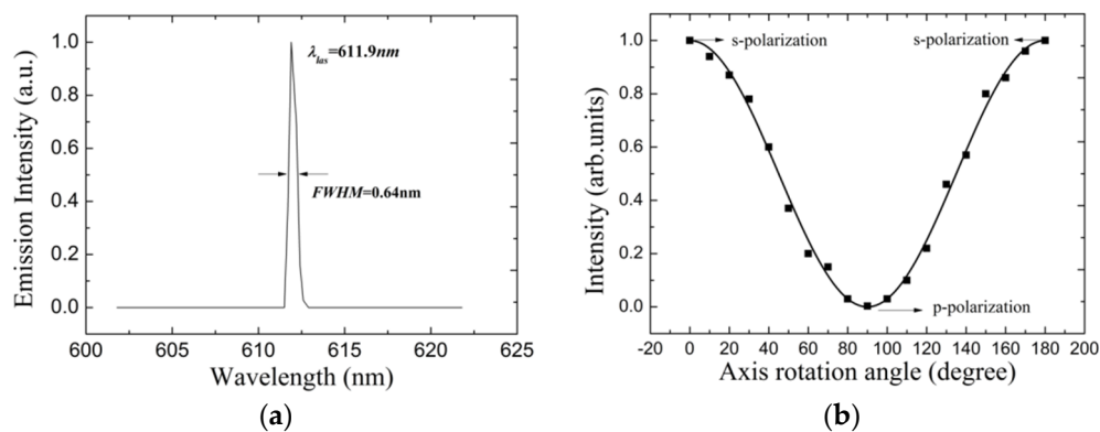
Figure 3. Lasing property of the 9th order HPDLC DFB laser. (a) Lasing spectra with the grating period selected at 1.72 \mu\text{m} and (b) the emission intensity as a function of the polarizer axis rotation angle.
