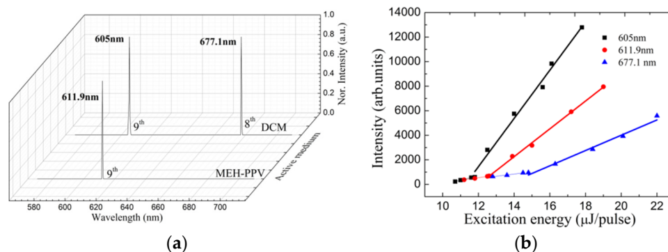
Figure 5. Tri-wavelength lasing property for the dye-doped HPDLC DFB laser at 20 °C. (a) Tri-wavelength lasing spectra of the dye-doped holographic polymer-dispersed liquid crystal (HPDLC)-distributed feedback (DFB) laser. The grating period was 1.72 \mu\text{m} for the tri-wavelength lasing operation. (b) Dependence of output emission intensity to excitation energy for different wavelength.
